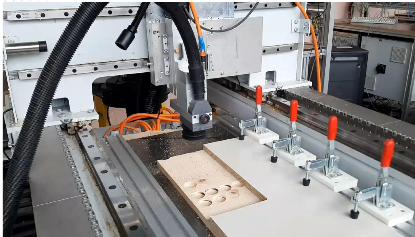
Milling of furniture parts – chipboard...
