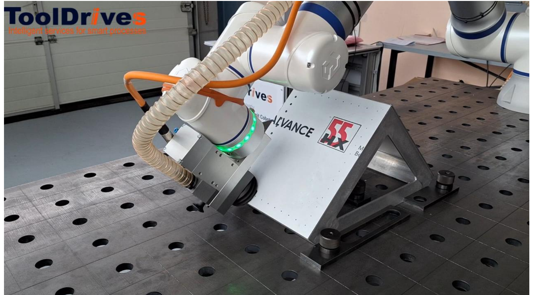
Drilling/Milling Alu - with Suction
