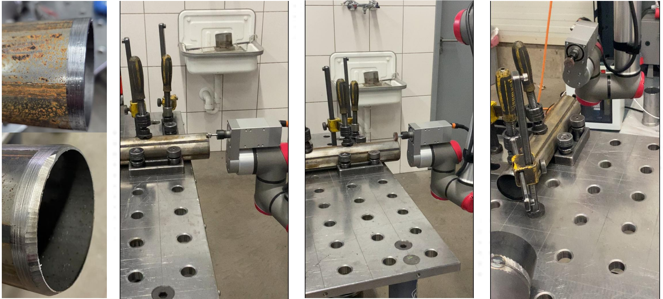
Beveling of steel pipes and removal of mill scale for welding preparation with UR10
