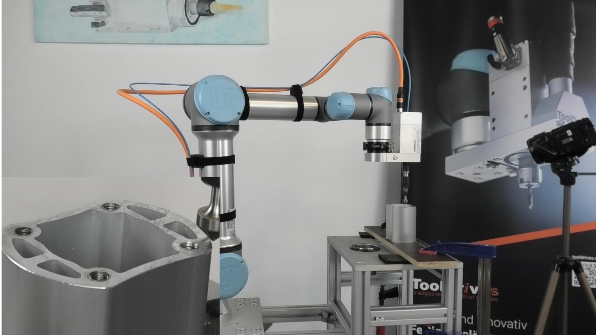
Deburring ALU
