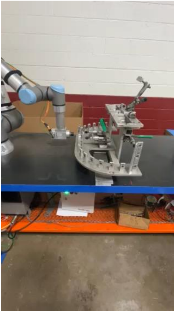
Drilling plastic with UR10e
